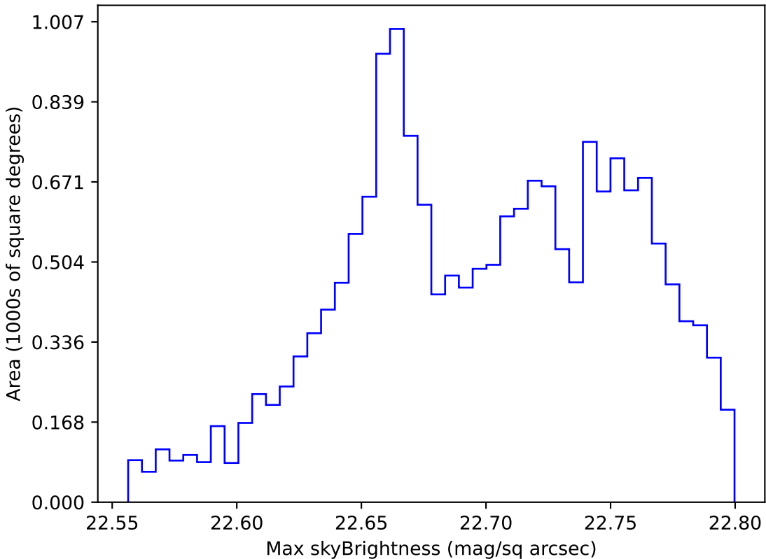
telescope_jerk_v3.5_10yrs WFD all bands: Max skyBrightness
