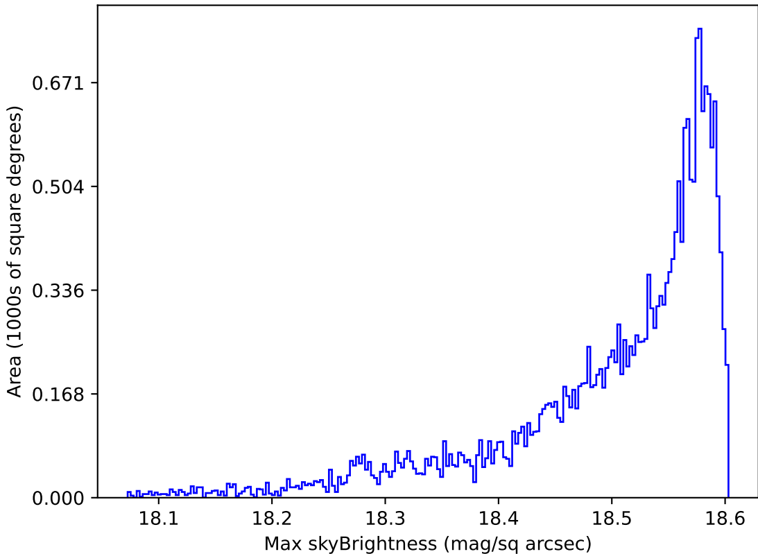
telescope_jerk_v3.5_10yrs All sky y band: Max skyBrightness
