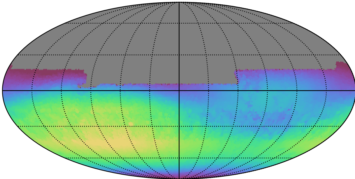
telescope_jerk_v3.5_10yrs All sky u band: Max skyBrightness
