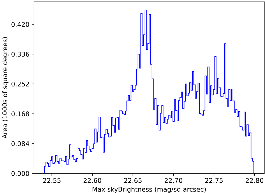
telescope_jerk_v3.5_10yrs All sky u band: Max skyBrightness
