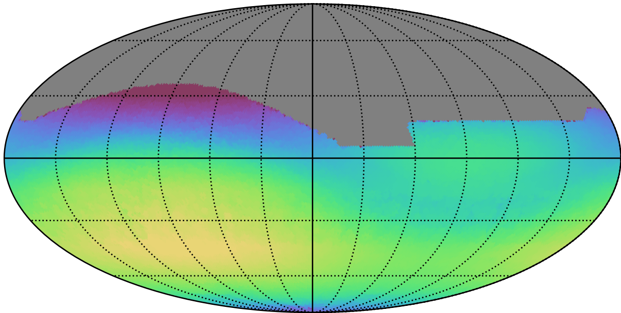
telescope_jerk_v3.5_10yrs All sky r band: Max skyBrightness
