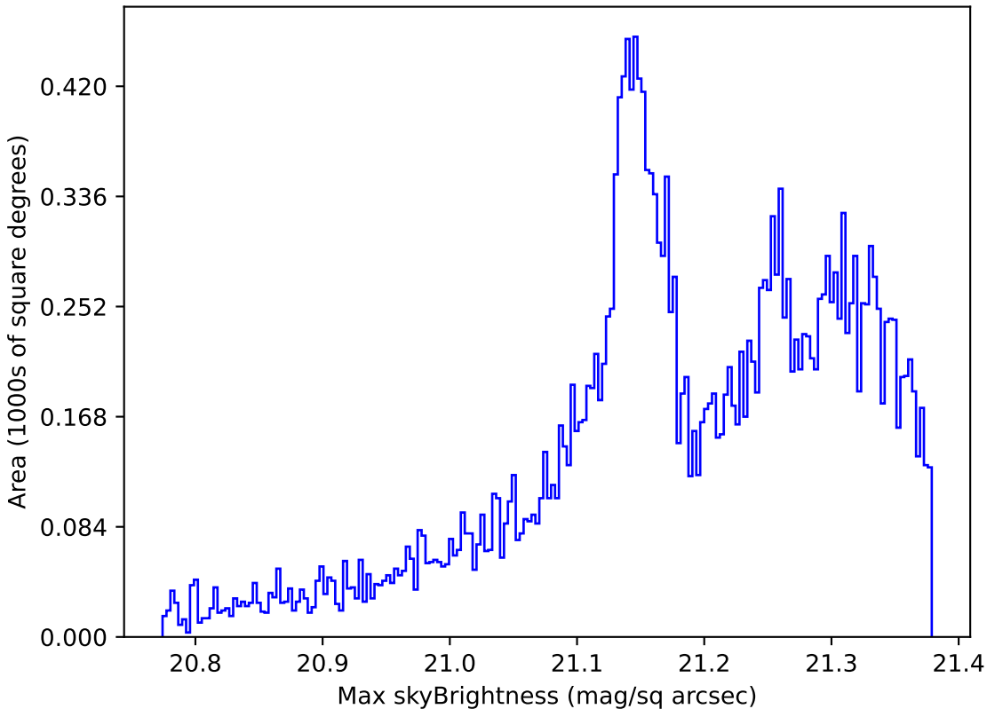
telescope_jerk_v3.5_10yrs All sky r band: Max skyBrightness
