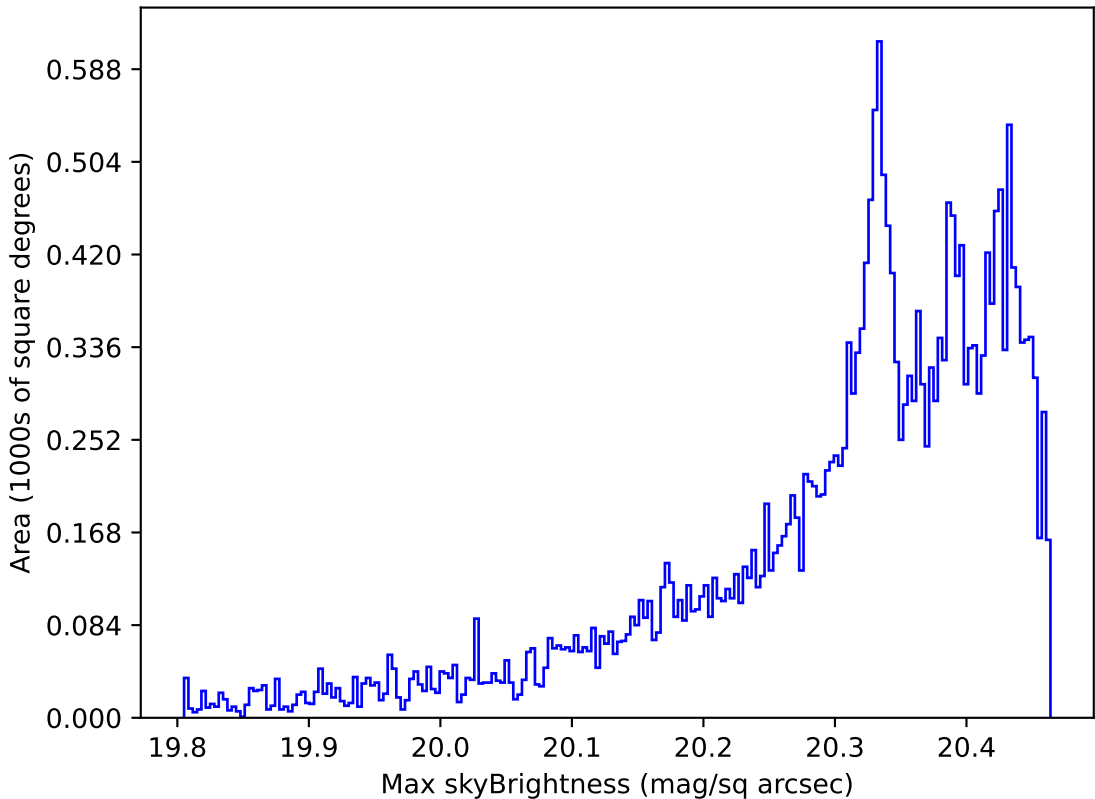
telescope_jerk_v3.5_10yrs All sky i band: Max skyBrightness
