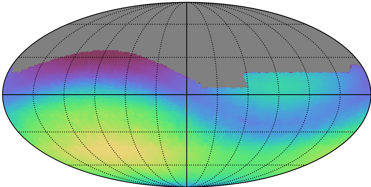
telescope_jerk_v3.5_10yrs All sky g band: Max skyBrightness
