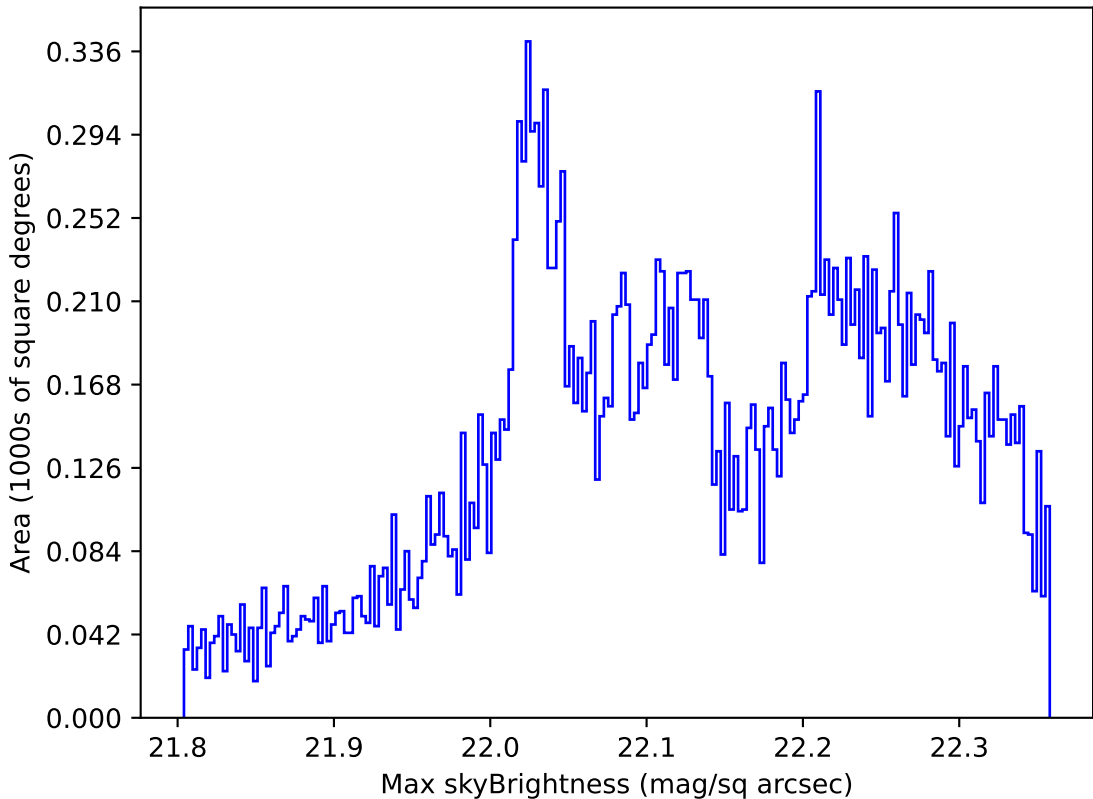
telescope_jerk_v3.5_10yrs All sky g band: Max skyBrightness
