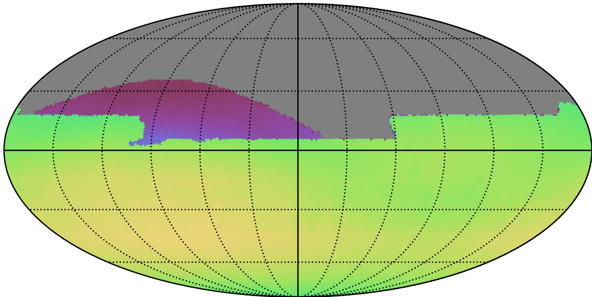
telescope_jerk_v3.5_10yrs All sky all bands: Max skyBrightness
