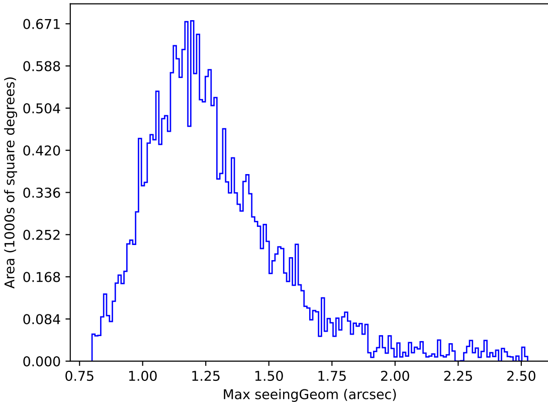
telescope_jerk_v3.5_10yrs Yr 1 z band: Max seeingGeom
