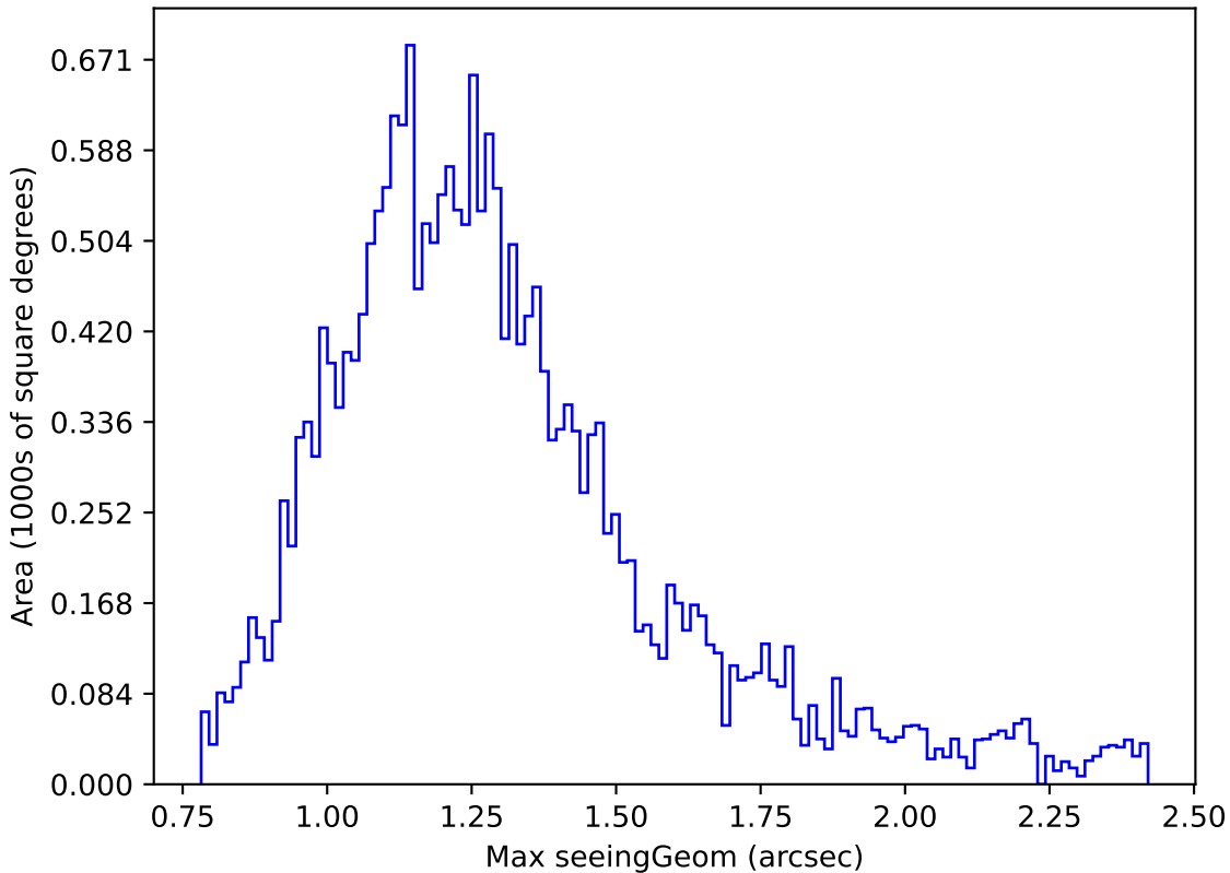
telescope_jerk_v3.5_10yrs Yr 1 y band: Max seeingGeom
