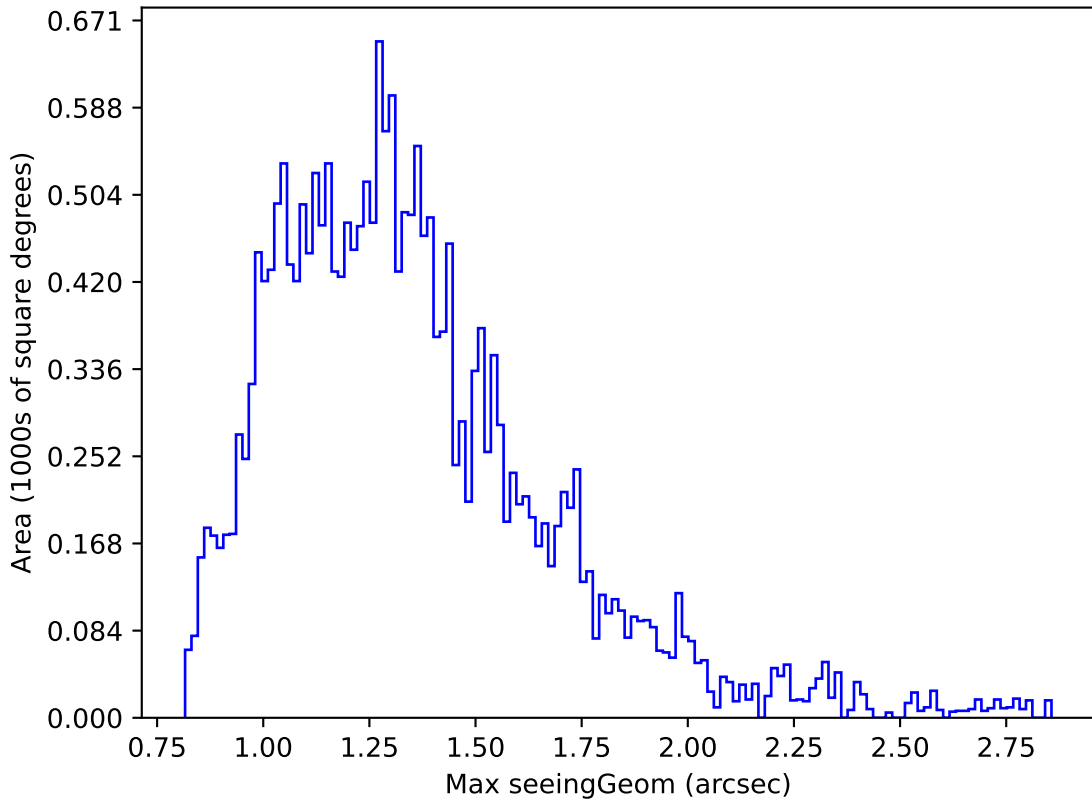
telescope_jerk_v3.5_10yrs Yr 1 u band: Max seeingGeom
