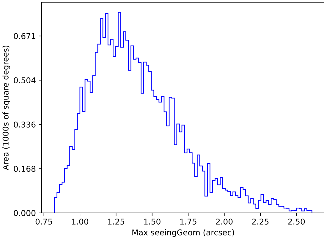
telescope_jerk_v3.5_10yrs Yr 1 r band: Max seeingGeom
