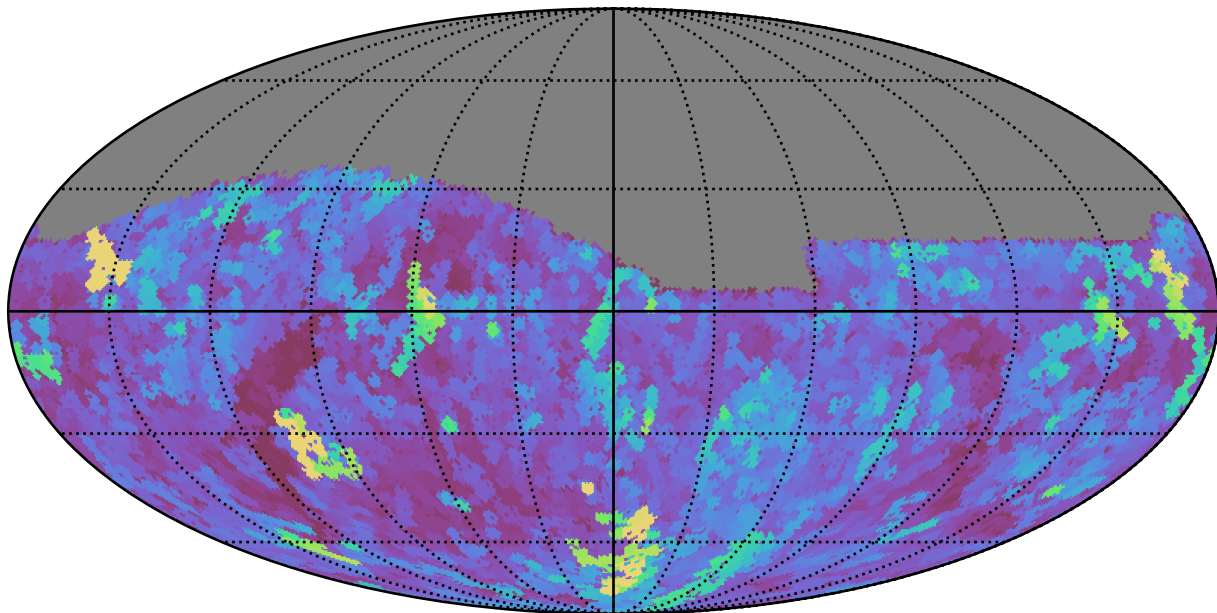
telescope_jerk_v3.5_10yrs Yr 1 i band: Max seeingGeom
