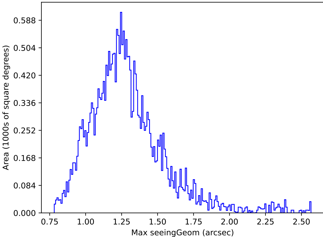
telescope_jerk_v3.5_10yrs Yr 1 i band: Max seeingGeom
