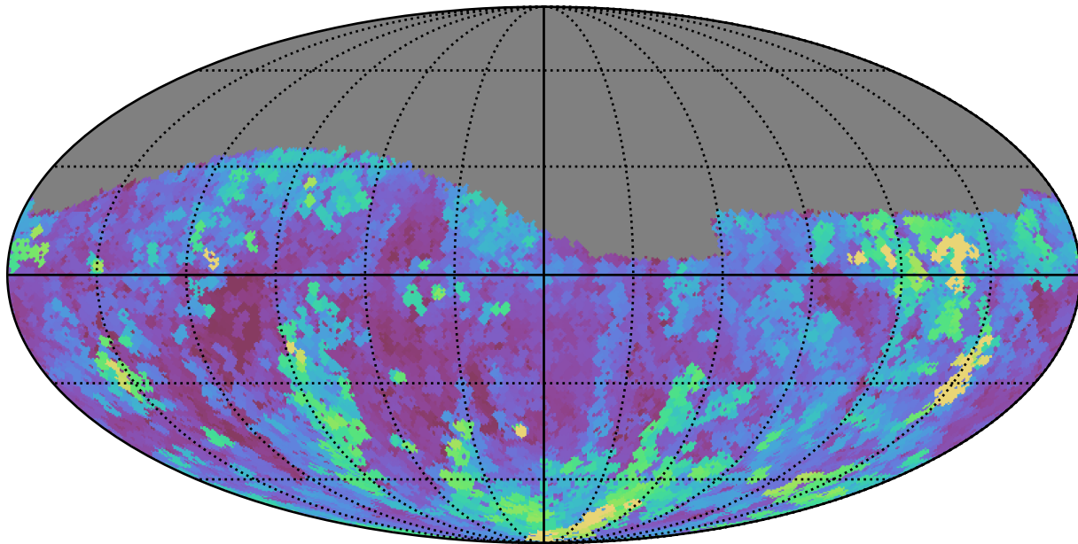
telescope_jerk_v3.5_10yrs Yr 1 g band: Max seeingGeom
