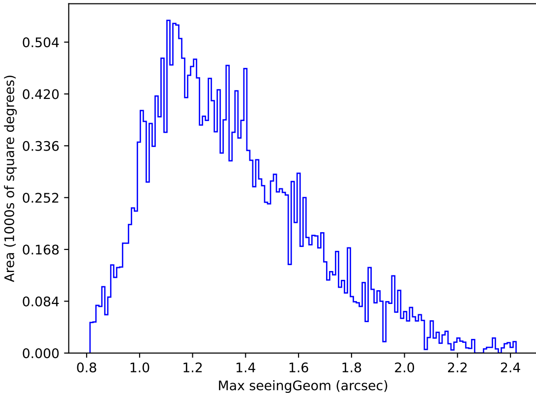
telescope_jerk_v3.5_10yrs Yr 1 g band: Max seeingGeom
