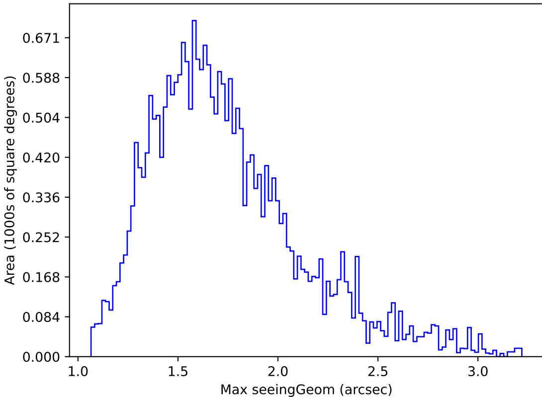
telescope_jerk_v3.5_10yrs Yr 1 all bands: Max seeingGeom
