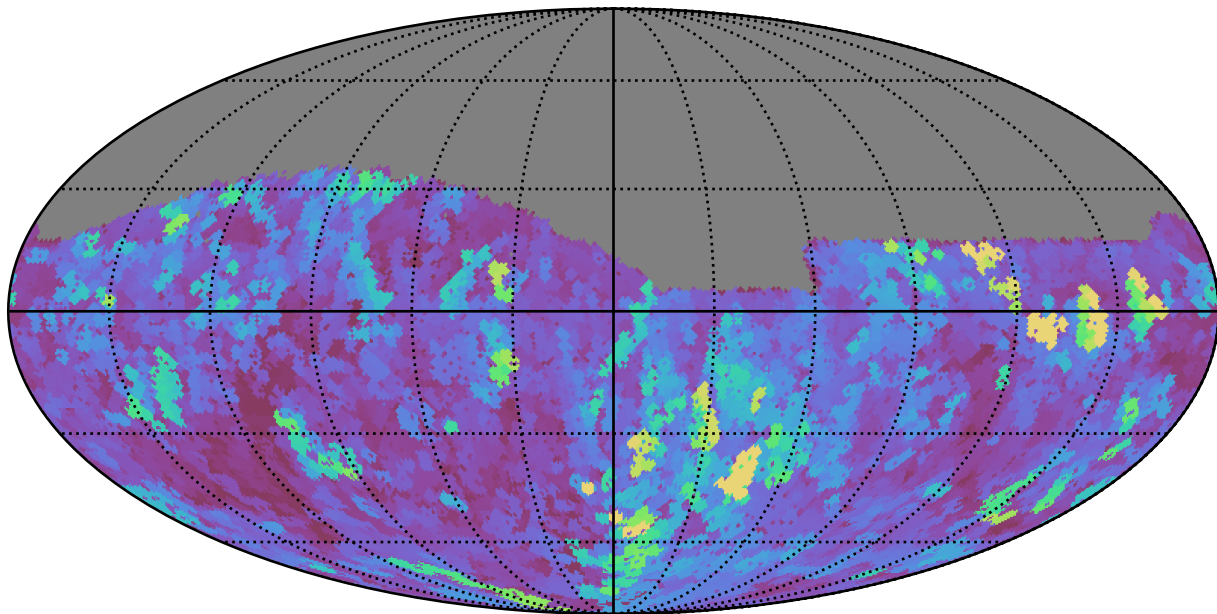
telescope_jerk_v3.5_10yrs Yr 1 z band: Max seeingEff
