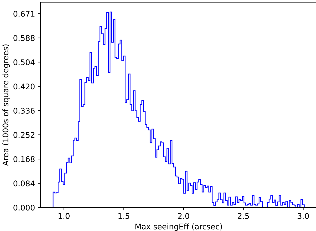
telescope_jerk_v3.5_10yrs Yr 1 z band: Max seeingEff
