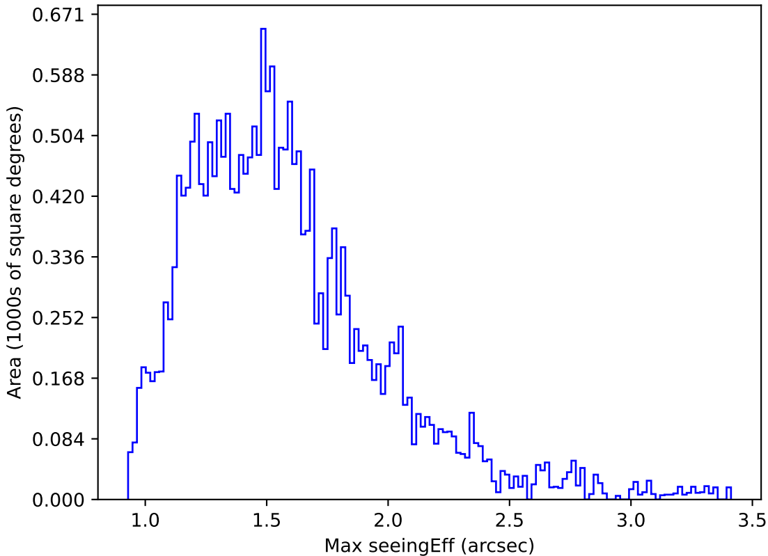
telescope_jerk_v3.5_10yrs Yr 1 u band: Max seeingEff
