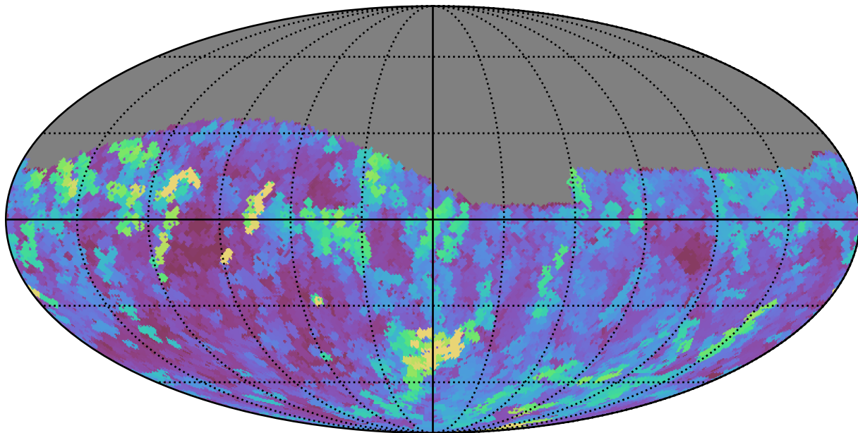
telescope_jerk_v3.5_10yrs Yr 1 r band: Max seeingEff
