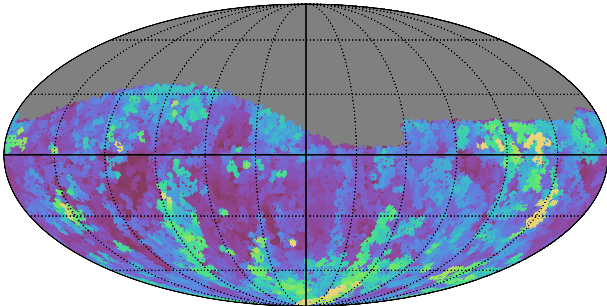
telescope_jerk_v3.5_10yrs Yr 1 g band: Max seeingEff
