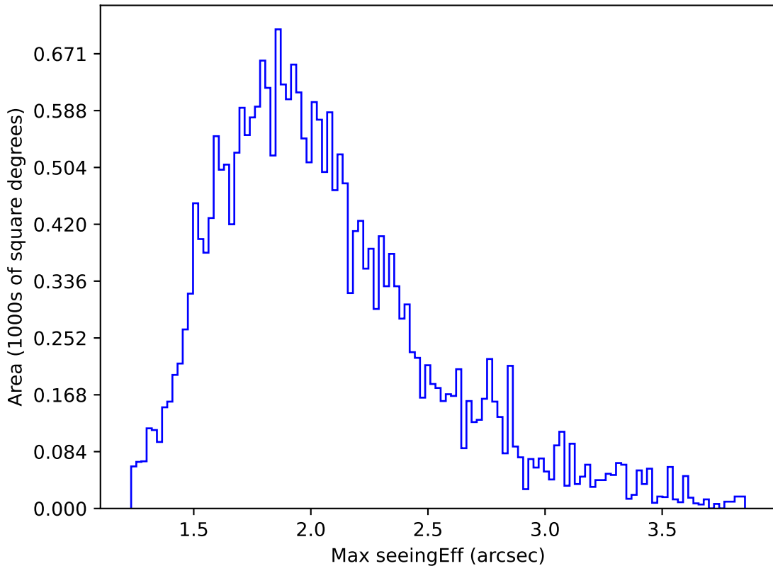
telescope_jerk_v3.5_10yrs Yr 1 all bands: Max seeingEff
