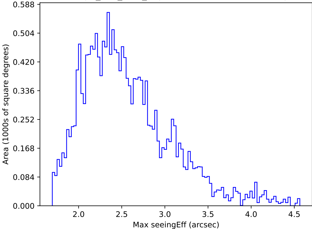
telescope_jerk_v3.5_10yrs WFD z band: Max seeingEff
