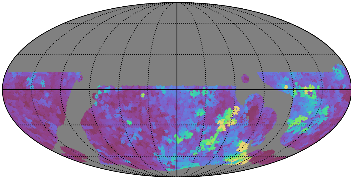
telescope_jerk_v3.5_10yrs WFD y band: Max seeingEff
