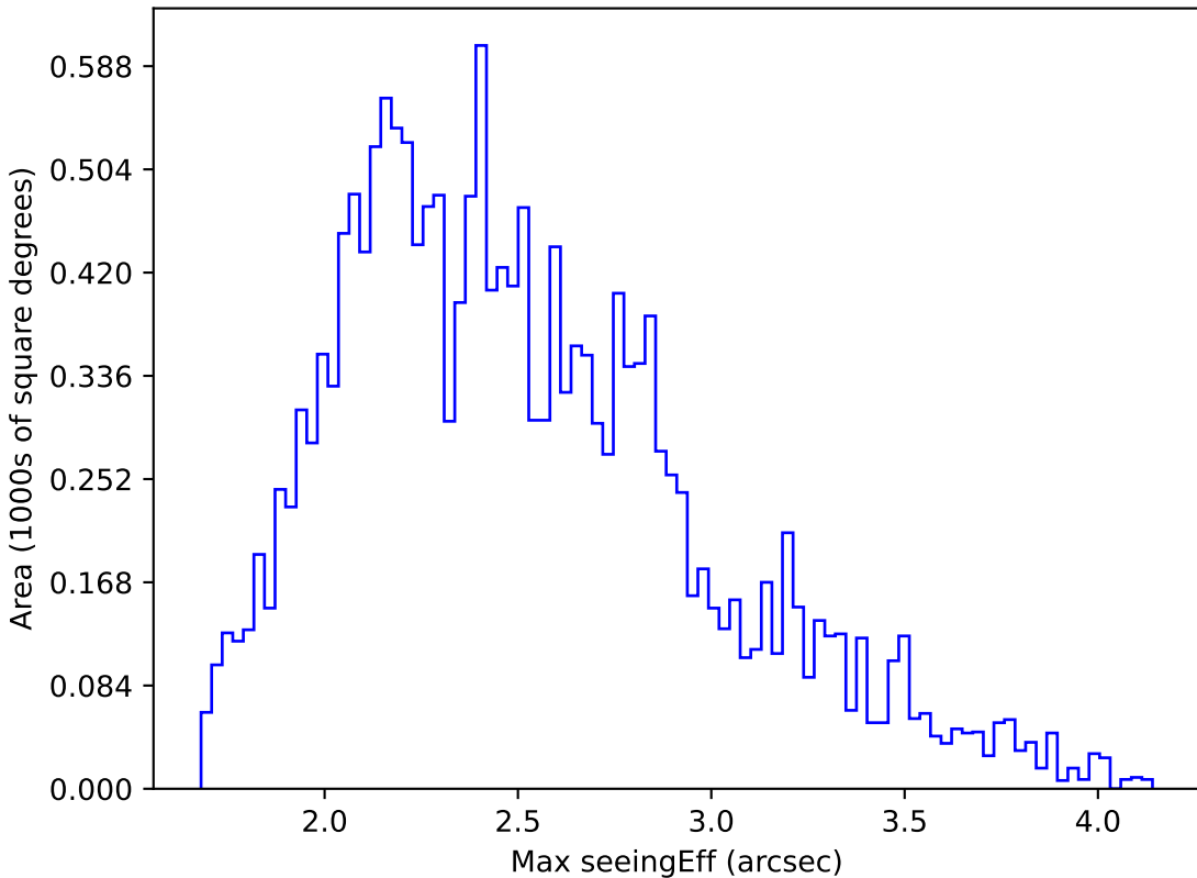
telescope_jerk_v3.5_10yrs WFD u band: Max seeingEff
