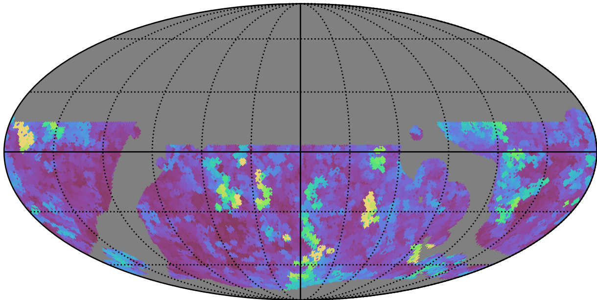
telescope_jerk_v3.5_10yrs WFD i band: Max seeingEff
