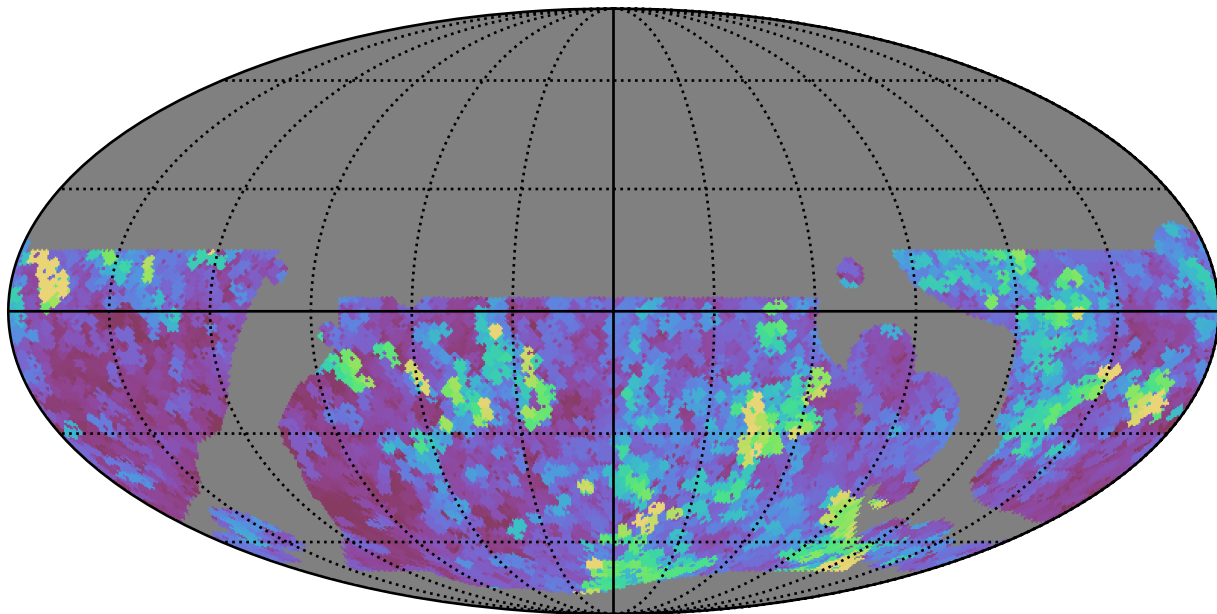
telescope_jerk_v3.5_10yrs WFD all bands: Max seeingEff
