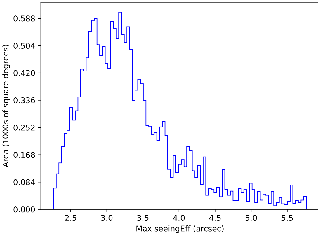
telescope_jerk_v3.5_10yrs WFD all bands: Max seeingEff
