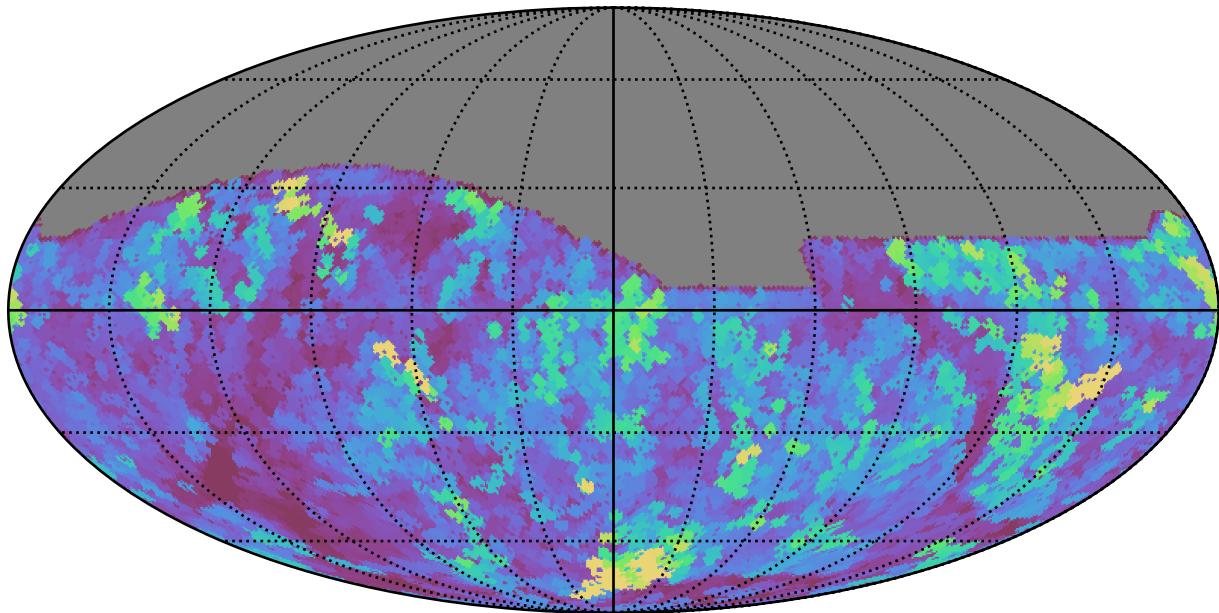
telescope_jerk_v3.5_10yrs All sky z band: Max seeingEff
