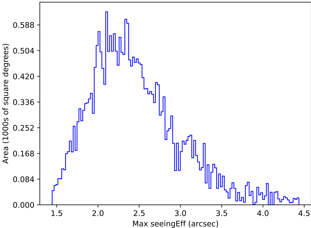
telescope_jerk_v3.5_10yrs All sky z band: Max seeingEff
