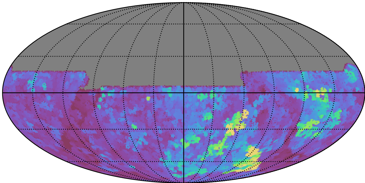
telescope_jerk_v3.5_10yrs All sky y band: Max seeingEff
