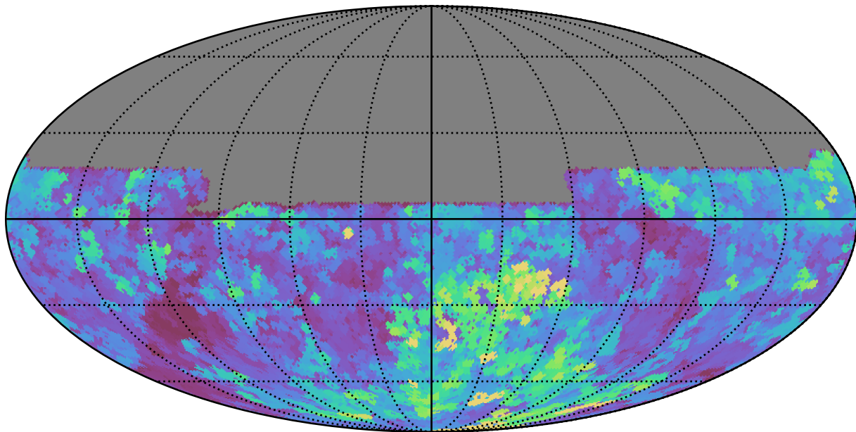
telescope_jerk_v3.5_10yrs All sky u band: Max seeingEff
