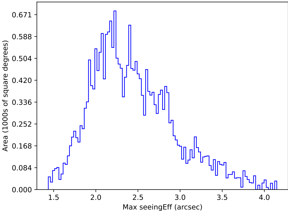
telescope_jerk_v3.5_10yrs All sky u band: Max seeingEff
