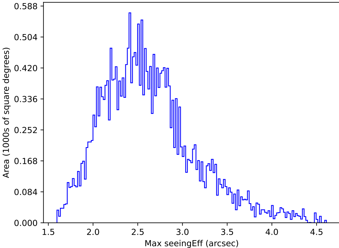
telescope_jerk_v3.5_10yrs All sky r band: Max seeingEff
