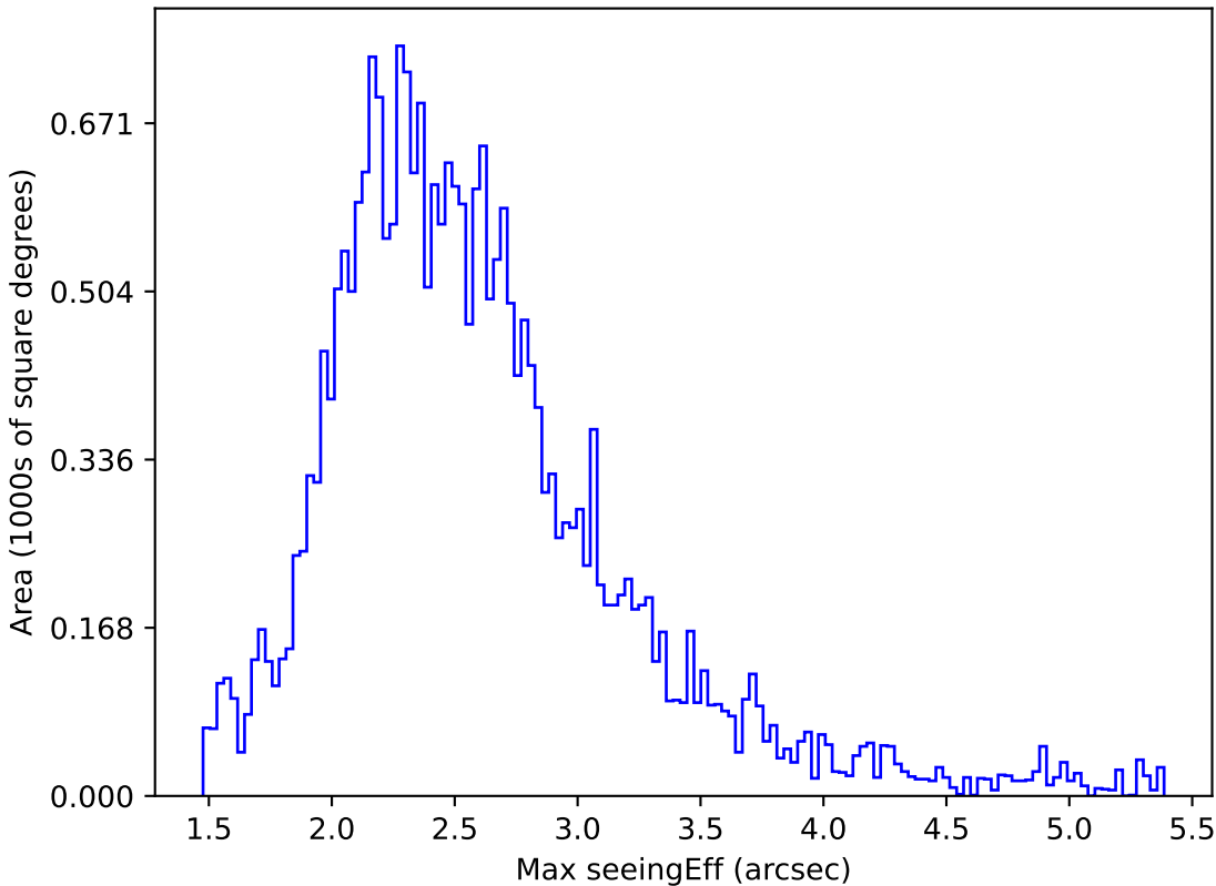
telescope_jerk_v3.5_10yrs All sky i band: Max seeingEff
