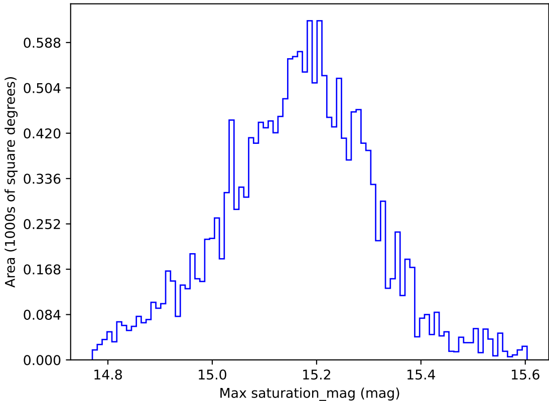
telescope_jerk_v3.5_10yrs WFD z band: Max saturation_mag
