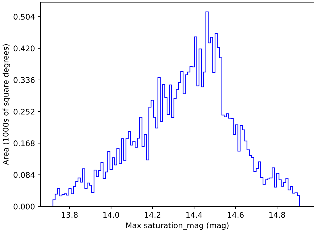
telescope_jerk_v3.5_10yrs WFD u band: Max saturation_mag
