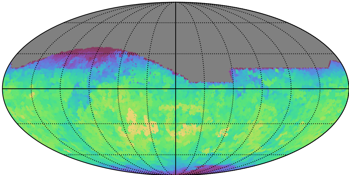
telescope_jerk_v3.5_10yrs All sky z band: Max saturation_mag
