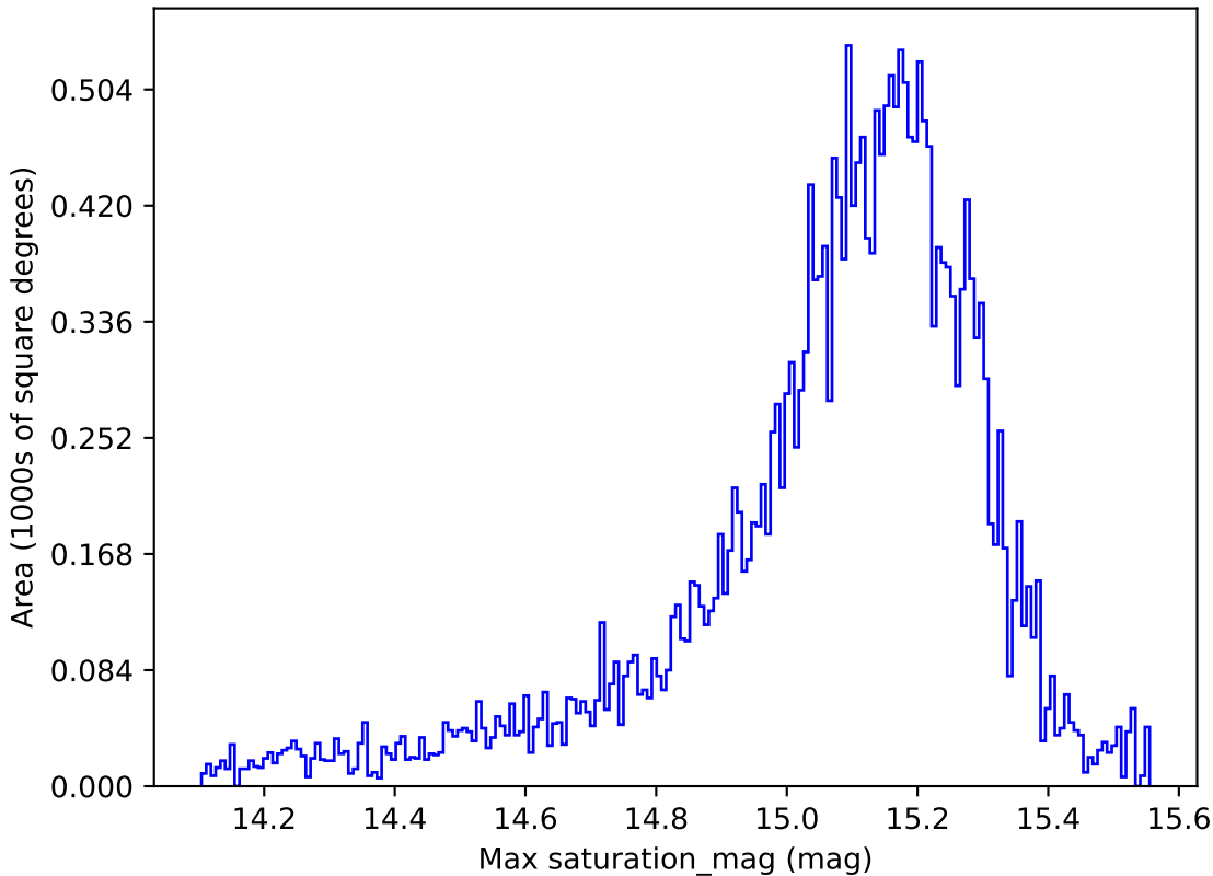
telescope_jerk_v3.5_10yrs All sky z band: Max saturation_mag
