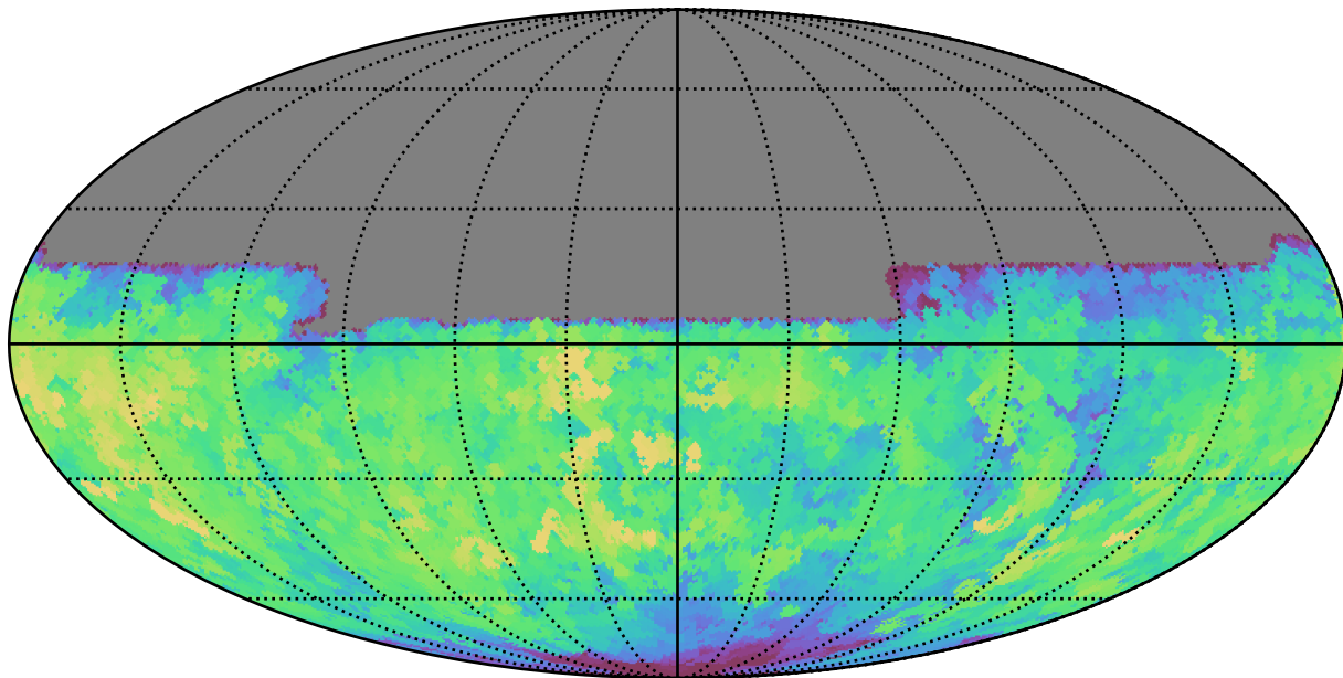
telescope_jerk_v3.5_10yrs All sky u band: Max saturation_mag
