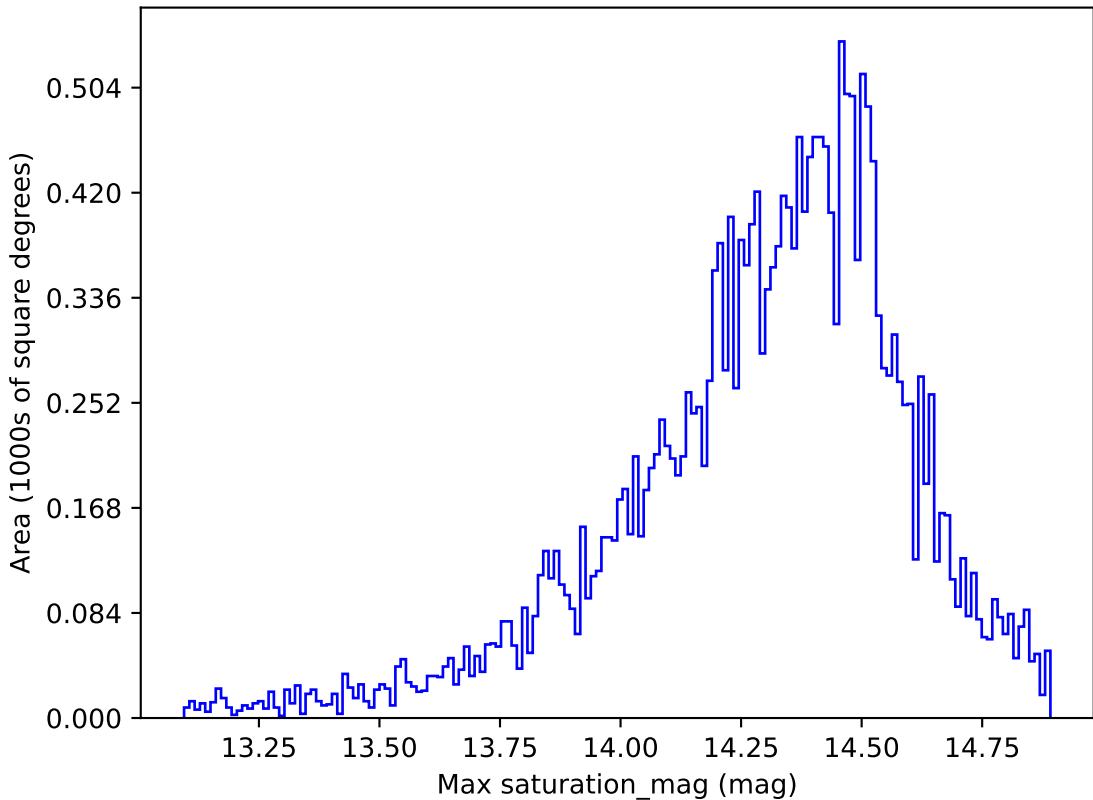
telescope_jerk_v3.5_10yrs All sky u band: Max saturation_mag
