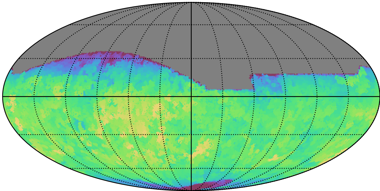
telescope_jerk_v3.5_10yrs All sky r band: Max saturation_mag
