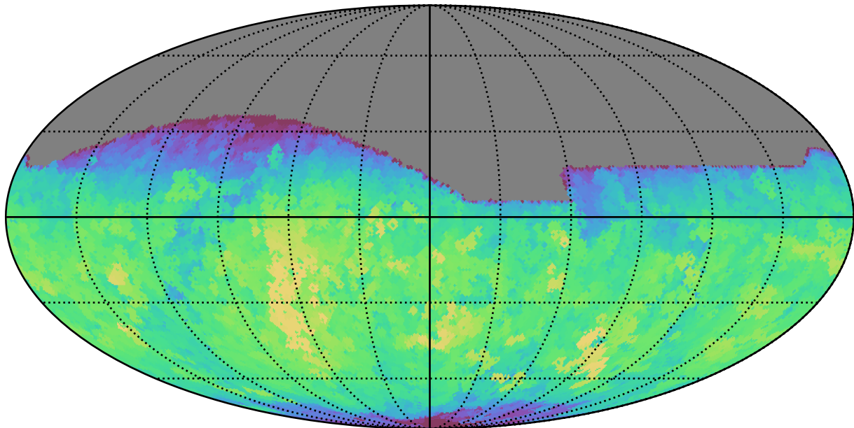
telescope_jerk_v3.5_10yrs All sky i band: Max saturation_mag
