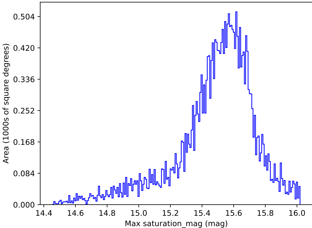
telescope_jerk_v3.5_10yrs All sky i band: Max saturation_mag
