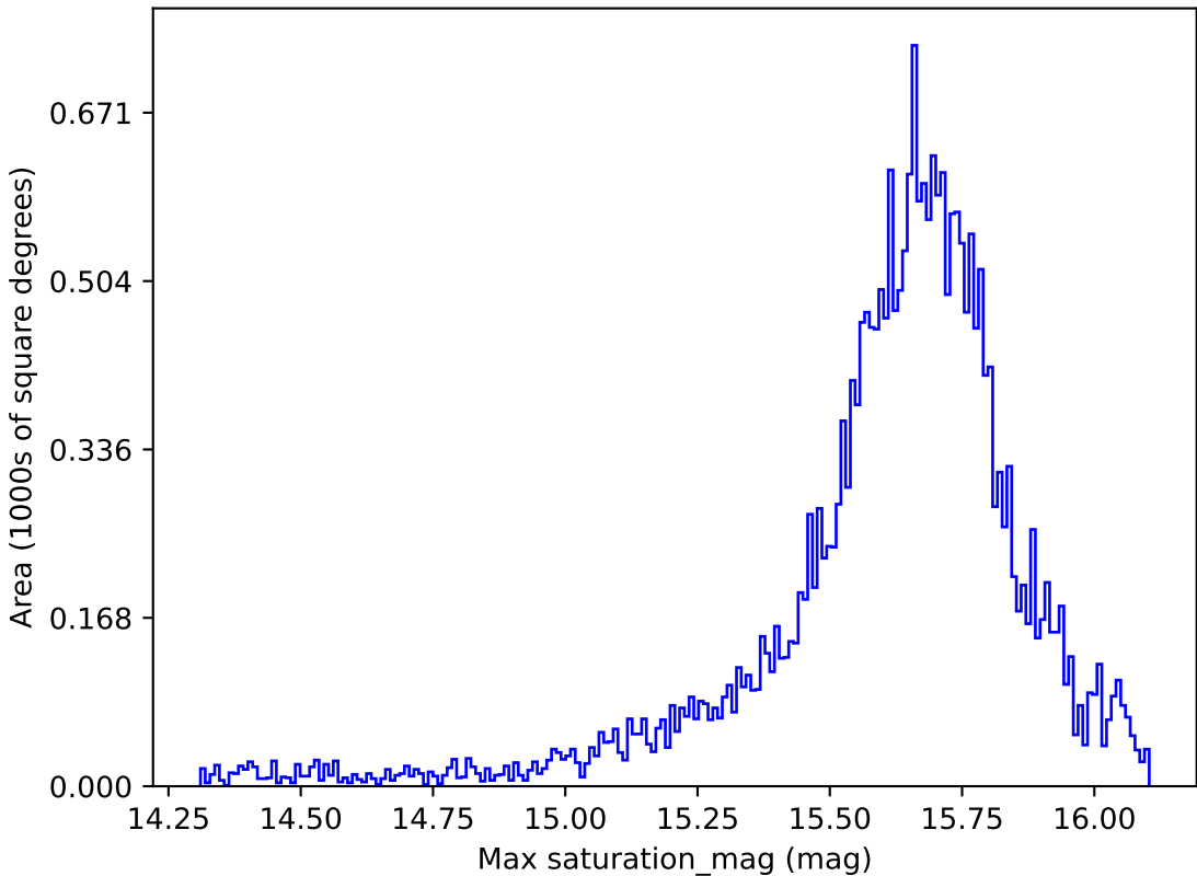
telescope_jerk_v3.5_10yrs All sky g band: Max saturation_mag
