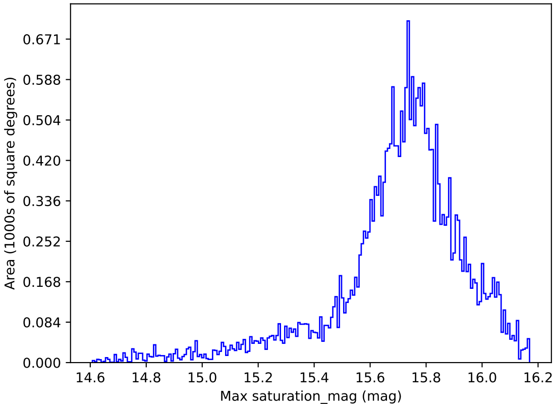
telescope_jerk_v3.5_10yrs All sky all bands: Max saturation_mag
