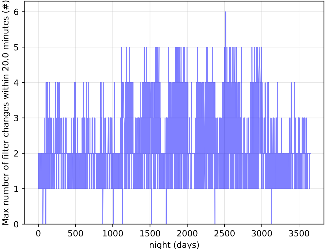
telescope_jerk_v3.5_10yrs Per Night: Max number of filter changes within 20.0 minutes
